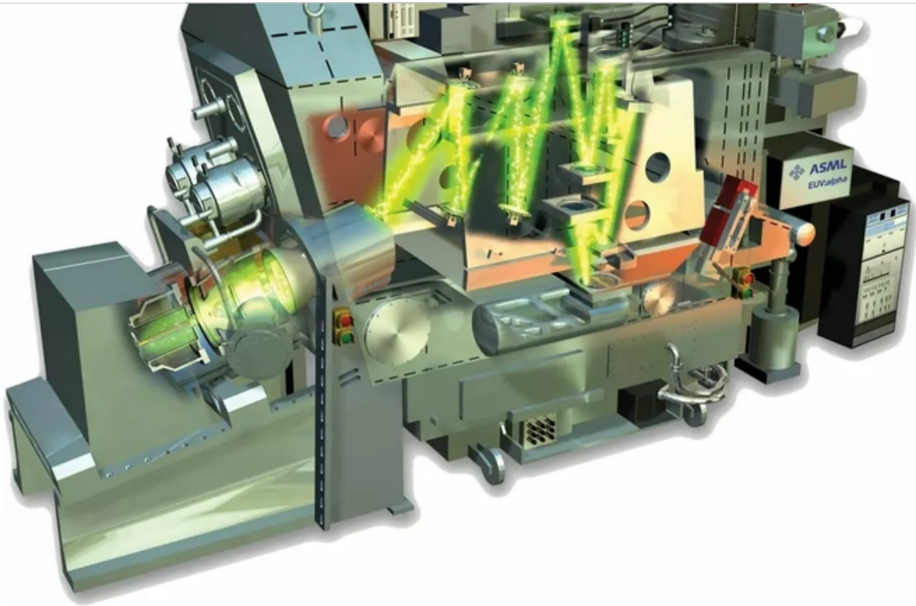
ASML's euv alpha-demotool
